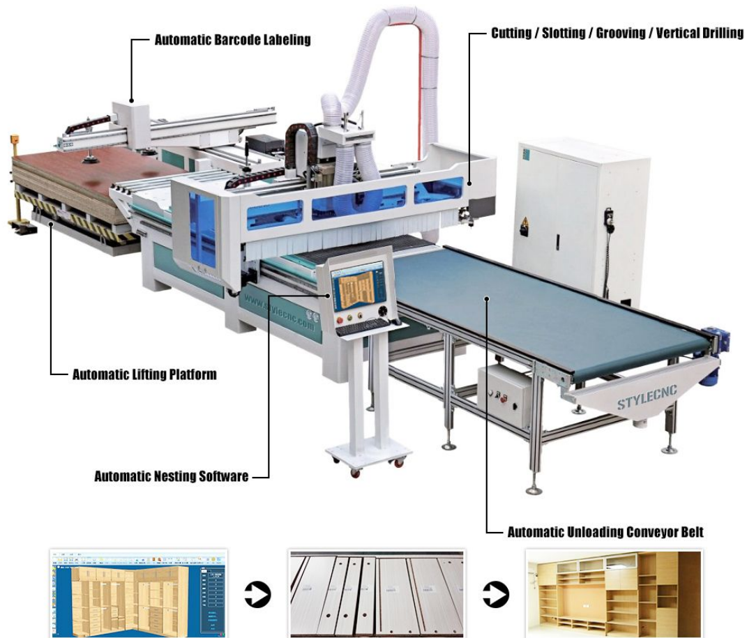
Intelligent Auto Nesting CNC Router S6
